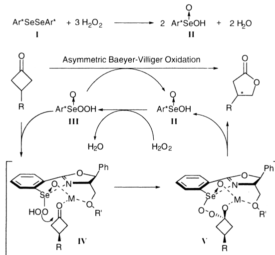
Scheme 2. Plausible pathway of asymmetric Baeyer–Villiger oxidation.
