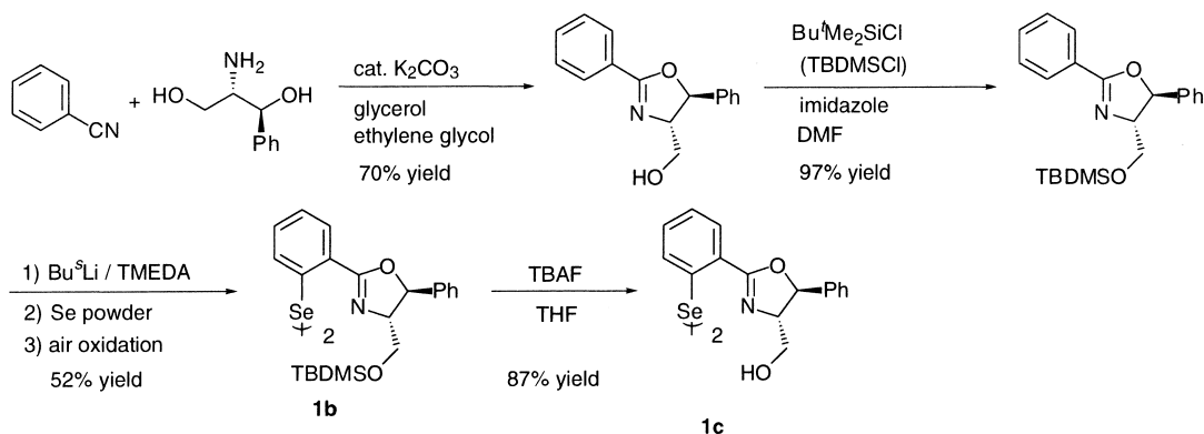
Scheme 1. Preparation of optically active diselenides.
