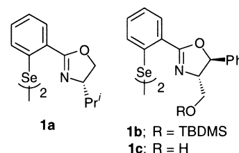
Chart 1. Optically active diselenides.
