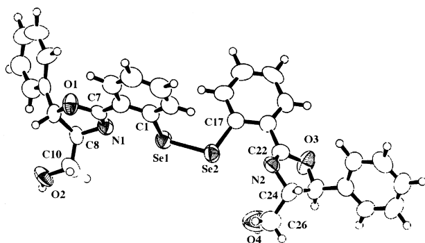
Fig. 1. The ORTEP drawing of optically active diselenide 1c . Selected bond lengths, angles, torsion angle ( \text{\AA} , deg): Se1–Se2 = 2.333(1); C7–N1 = 1.25(1); C22–N2 = 1.22(1) O1–C7–N1 = 119.5(8); O3–C22–N2 = 119.4(10); C1–Se1–Se2–C17 = –85.7(4).
